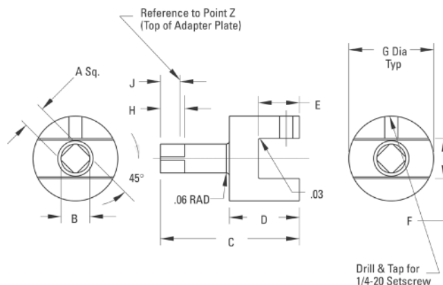
Ball Valve Drive Coupling
